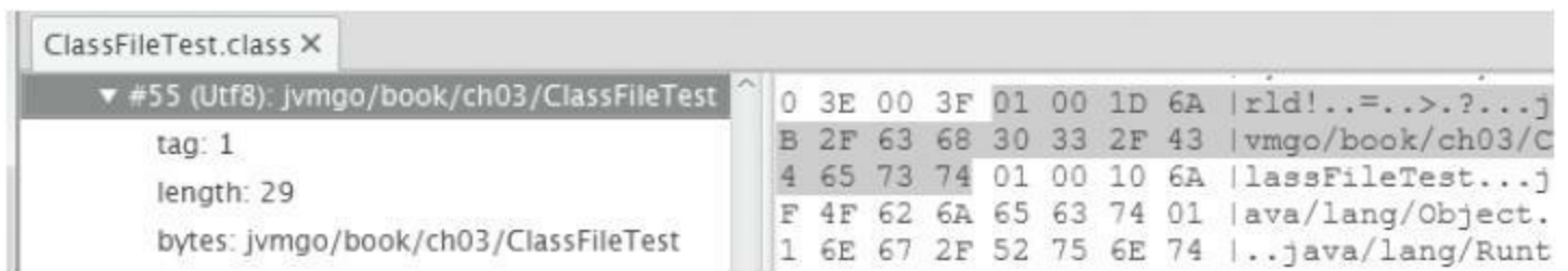
图3-17 用classpy观察CONSTANT_Class_info常量(2)
