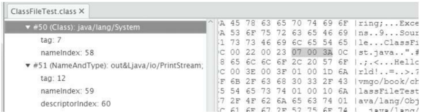
图3-19 用classpy观察CONSTANT_Fieldref_info常量(2)
